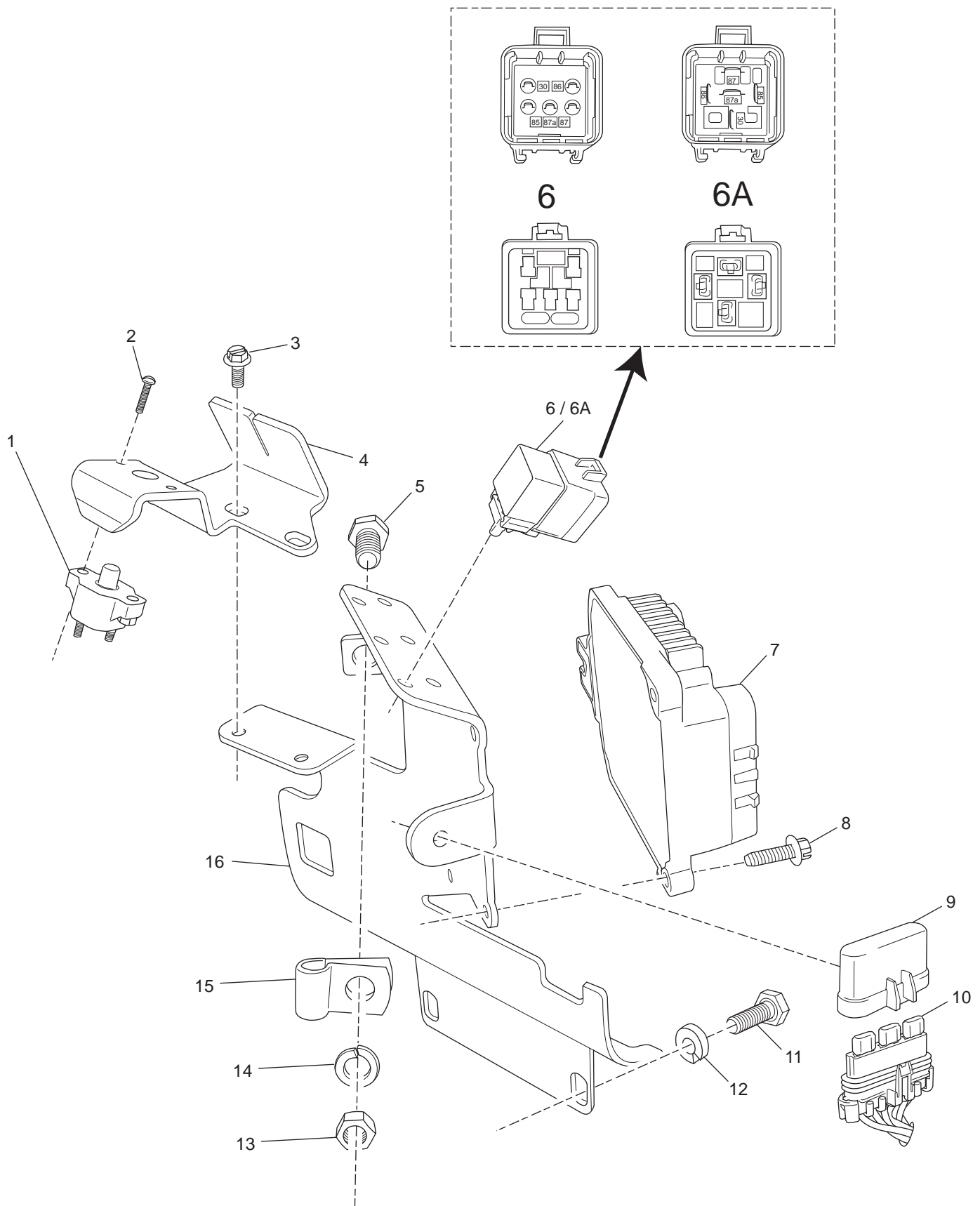
ECM and RELAYS - FIGURE 19
