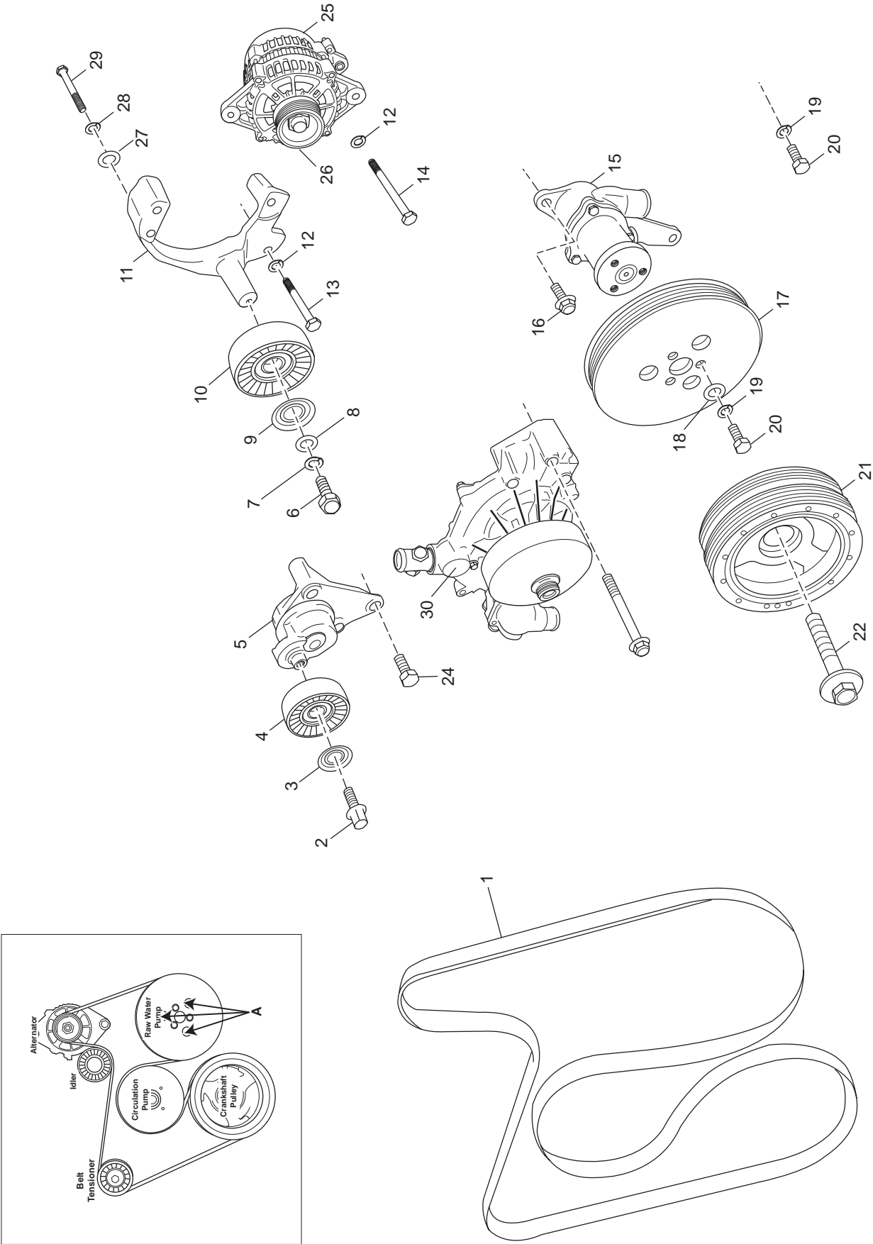
ACCESSORY DRIVE SYSTEM COMPONENTS - FIGURE 20
