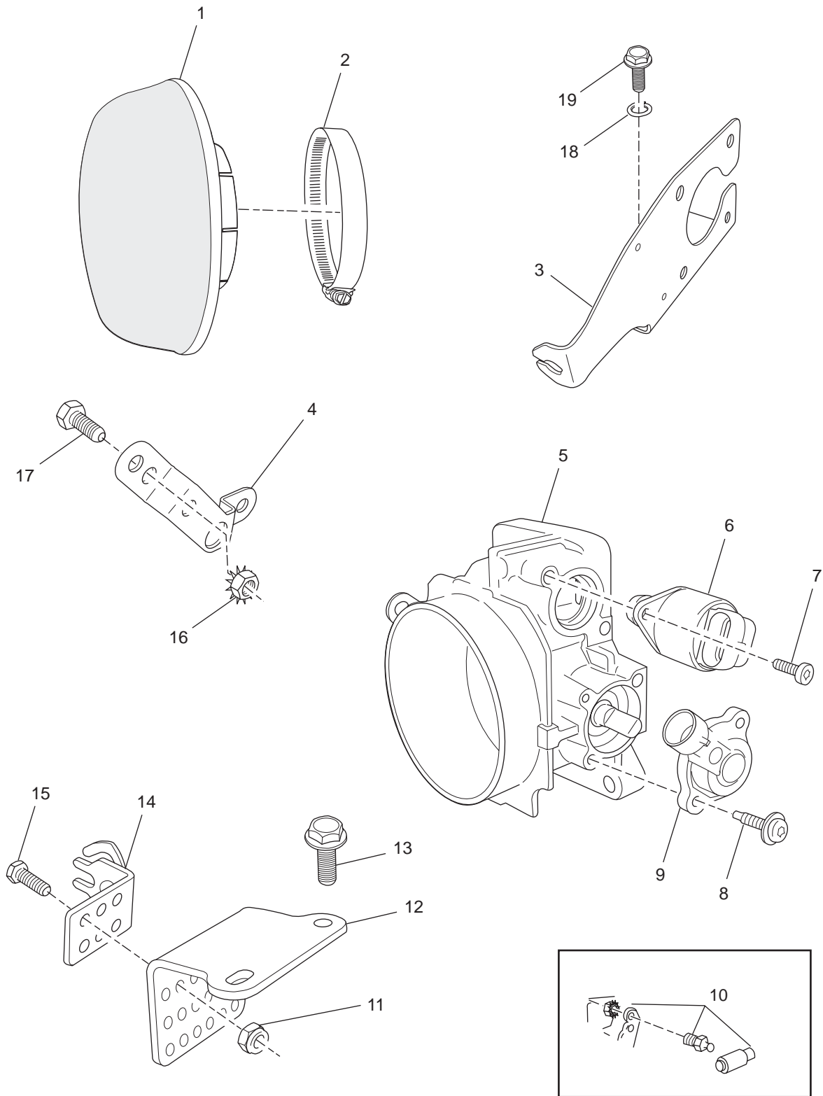
THROTTLE BODY and RELATED COMPONENTS - FIGURE 6
